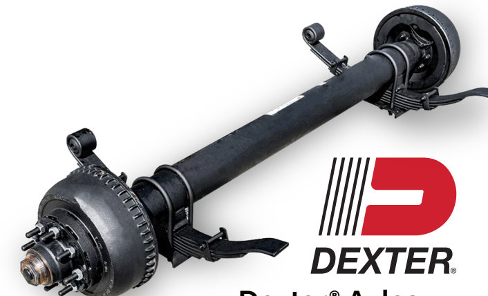
Dexter® Axles with Self-Adjusting Brakes
