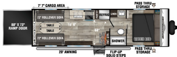
UUV - 5,400 | Exterior Length - 30'10" | Sleeps - 6
