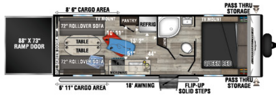
UUV - 5,300 | Exterior Length - 29'1" | Sleeps - 6
