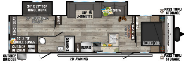
332BHKSE UUV - 7,390 | Exterior Length - 37'3" | Sleeps - 10
