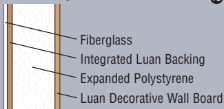
Wall Cut-Away
