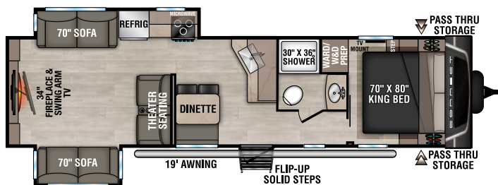
C312RE UVW - 7,790 | Exterior Length - 36'1" | Sleeps - 6
