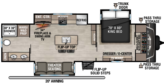
C293RB UVW - 8,210 | Exterior Length - 34' | Sleeps - 3
