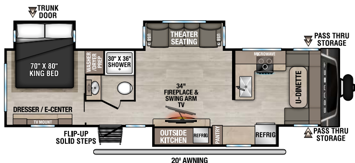
C323MCK UVW - 8,680 | Exterior Length - 37'1" | Sleeps - 5
