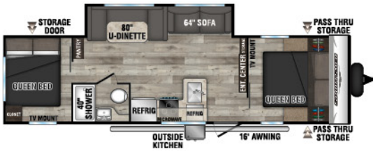
301DBSE UWW - 6,150 | Exterior Length - 32'10" | Sleeps - 8
