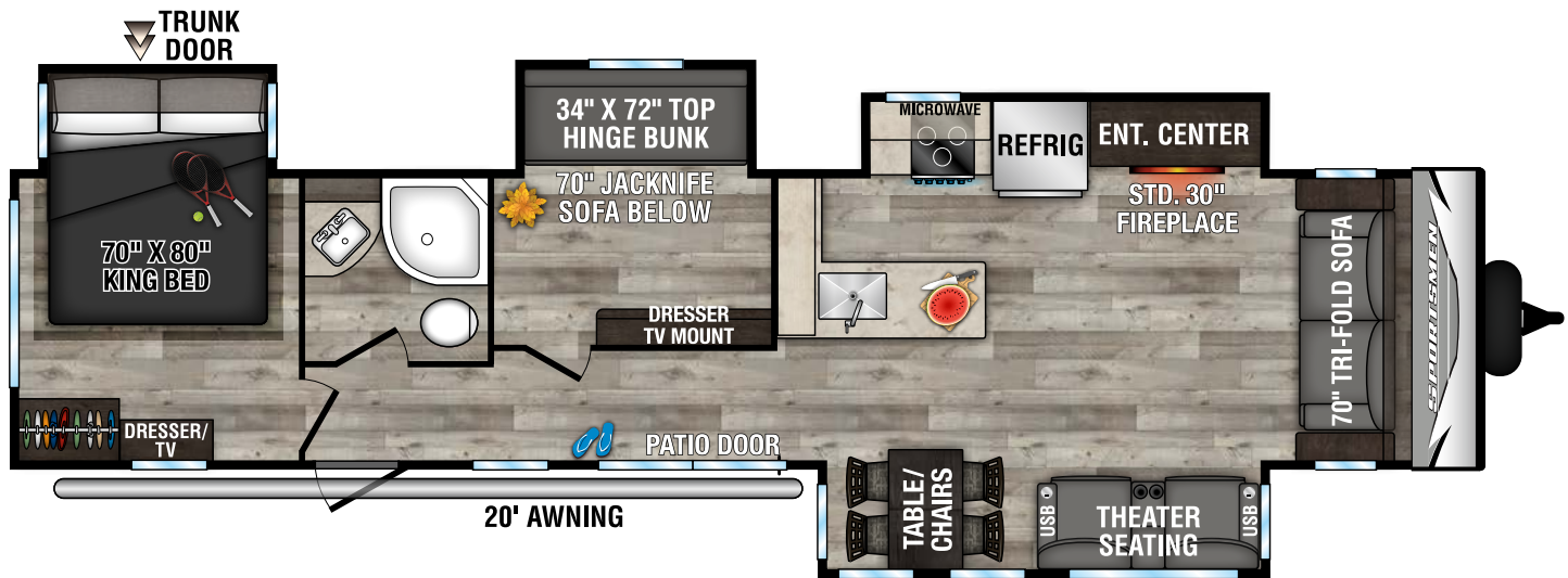
364BH UVW - 9,400 | Exterior Length - 41' 2" | Sleeps - 6
