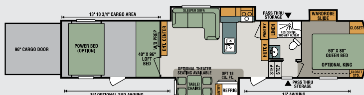
V4114TK UVW 14,400 • Dry Hitch Wt. 3,130 NCC 4,600 • Length 43' 4"
