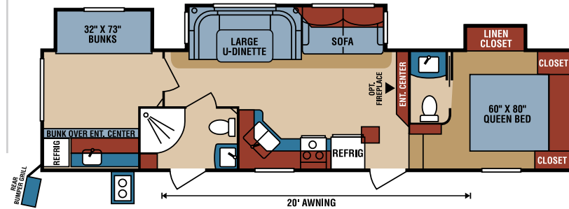
D292BHT UVW 9,430 • Dry Hitch Wt. 1,410 • NCC 2,070 • GVWR 11,500 • Length 35' 11"
