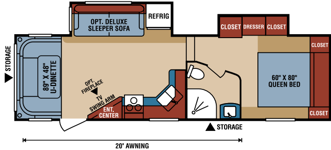
D259RDD UVW 7,600 Dry Hitch Wt. 1,200 NCC 2,400 GVWR 10,000 Length 29' 11"
