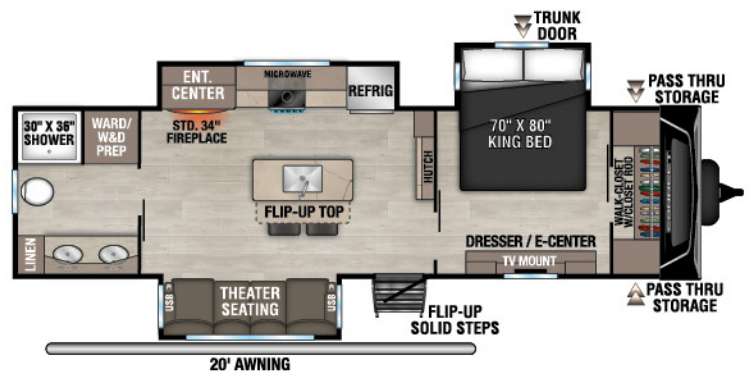
NEW C293RB UVW - 8,060 | Exterior Length - 34' | Sleeps - TBD
