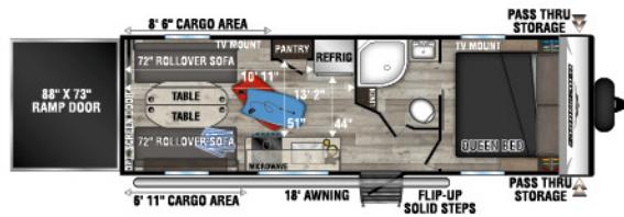
250THSE - TOY HAULER
