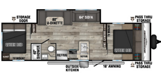
301DBSE UUV - 6,150 | Exterior Length - 32'10" | Sleeps - 8
