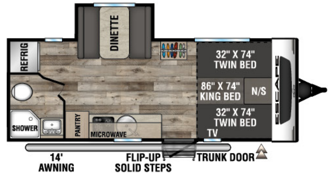
E201TB UYW - 3,520 | Exterior Length - 23' 9" | Sleeps - 3
