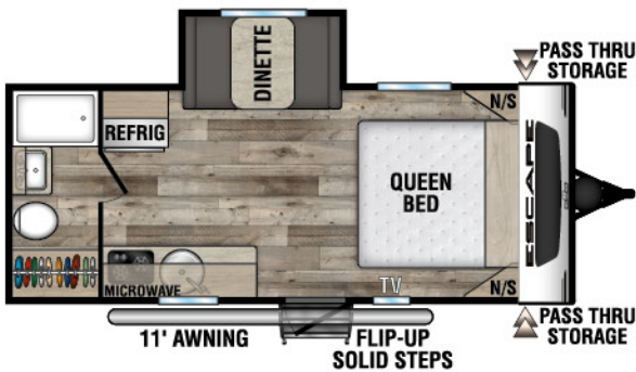
E181RB UVW - 3,270 | Exterior Length - 22'1" | Sleeps - 3
